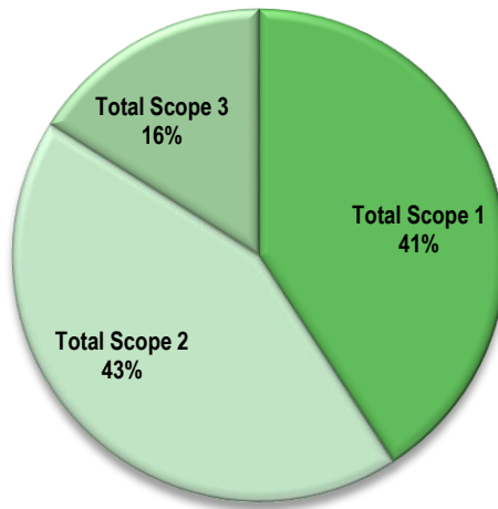
Figure 2: Total GHG emissions for Durban by scope (eThekweni Municipality, 2014b)
