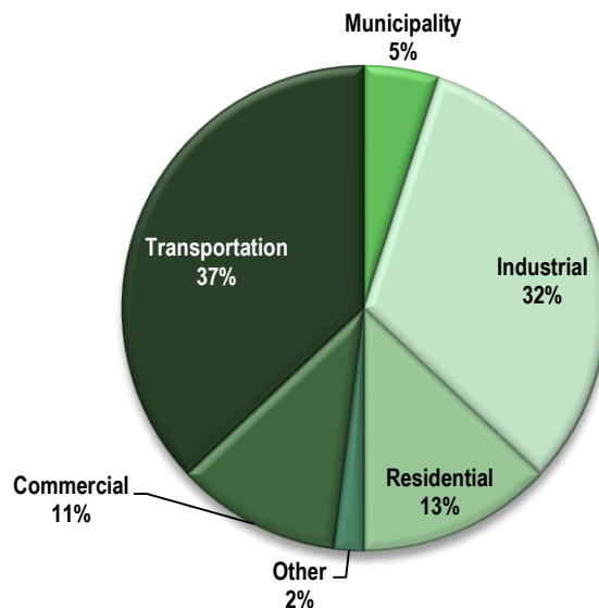
Figure 3: Total GHG emissions for Durban by sector (eThekweni Municipality, 2014b)
